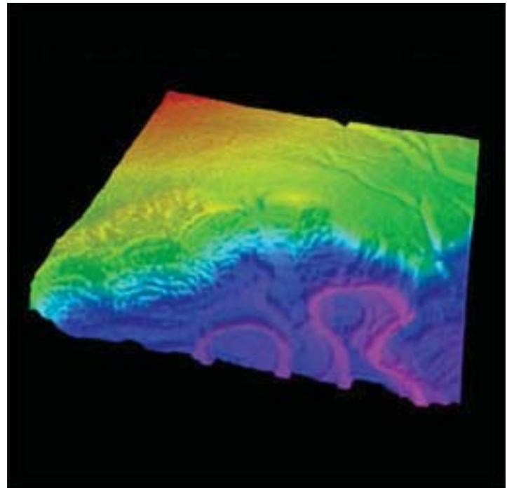
LIDAR representation from Jackson and Wyoming Counties
