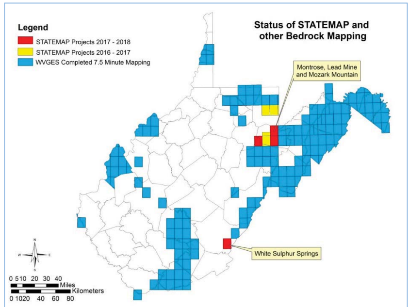
Status of STATEMAP bedrock mapping projects in West Virginia for Fiscal Year 2017
