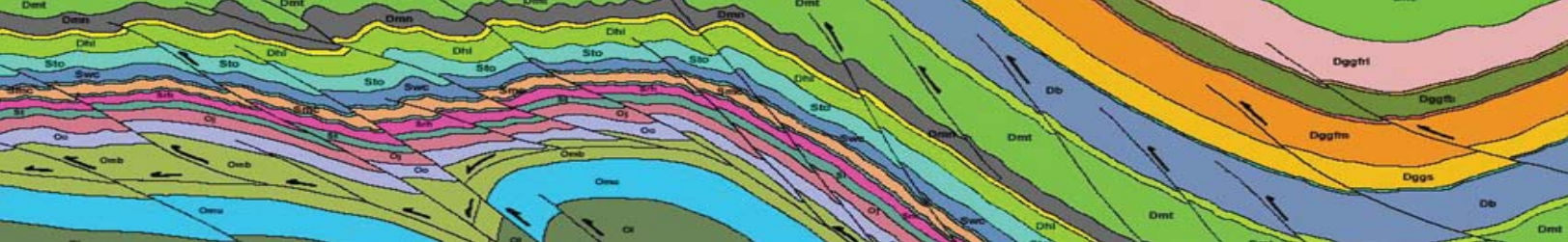
Portion of the Moorefield quadrangle's geologic cross section
